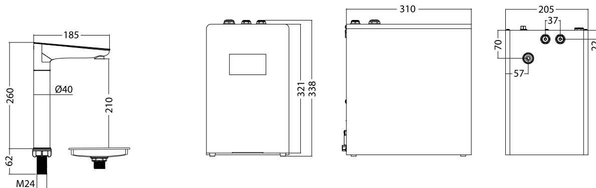
(Hot Water Unit 热水机)
