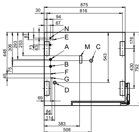
Connection points
